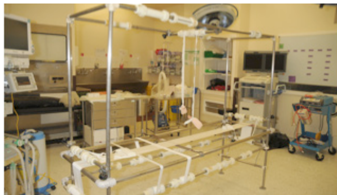
Figure 1. Plaster jacket application frame
